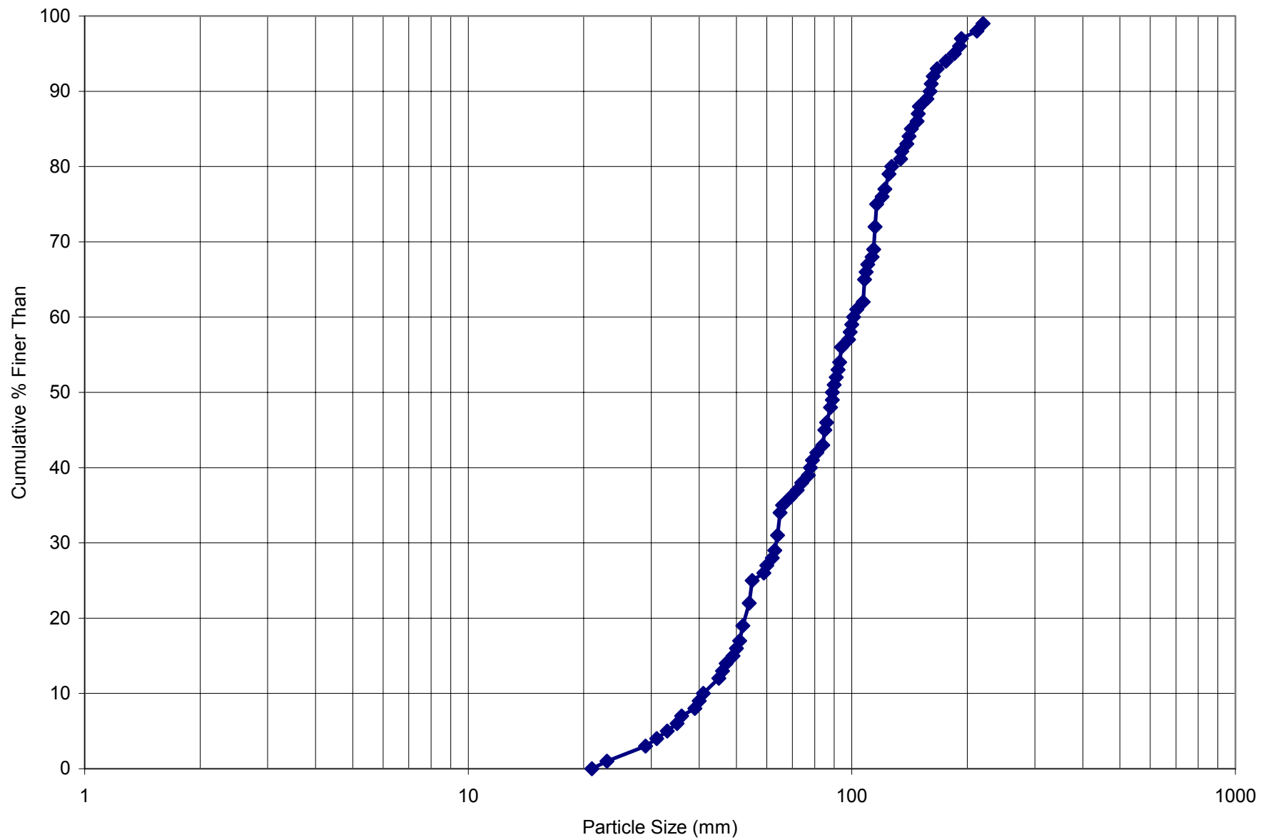
Figure B-5. Snelling site pebble count 3B.
